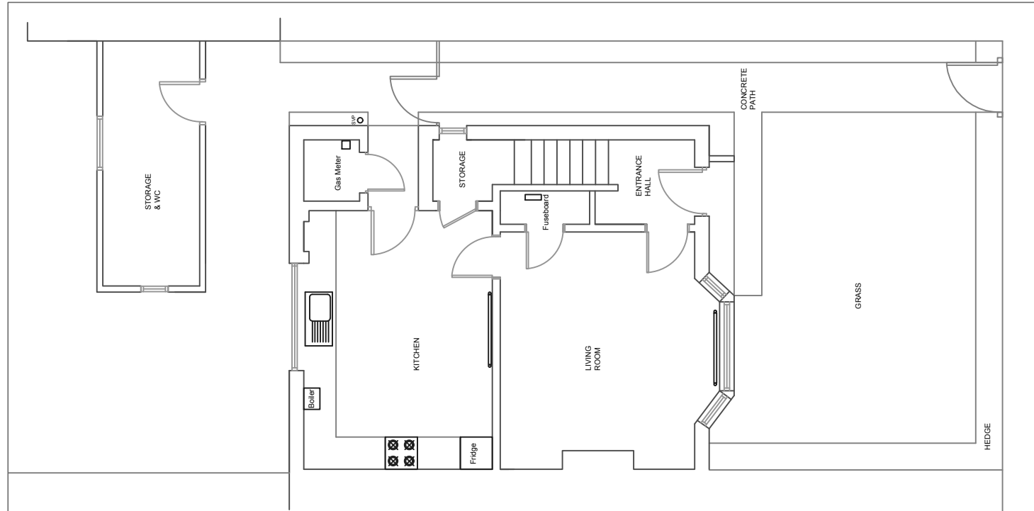
EXISTING GROUND FLOOR LAYOUT (1:100)
