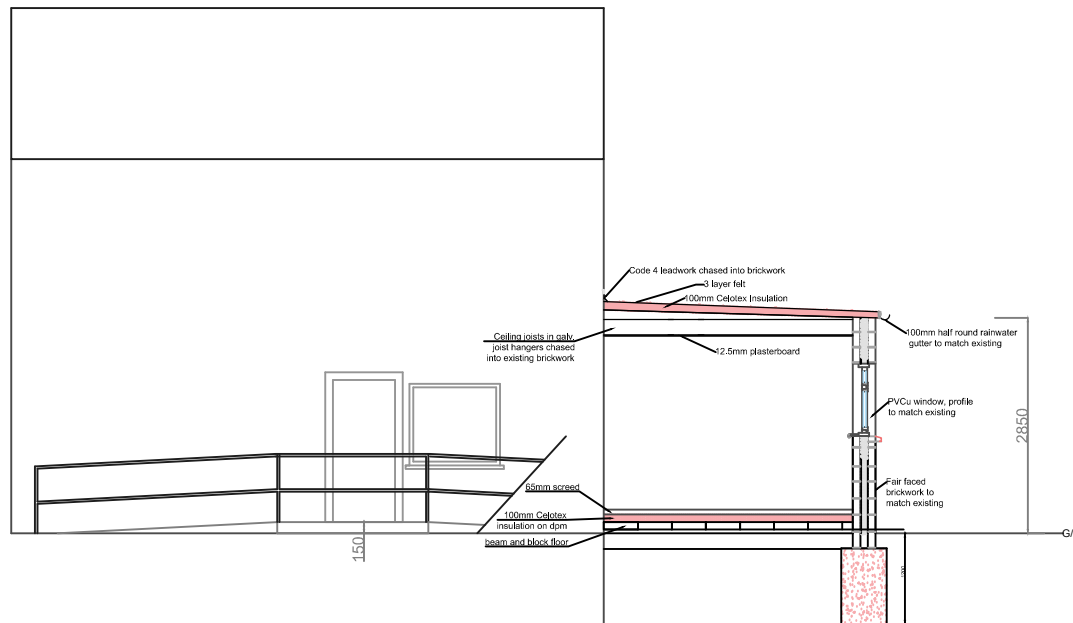
PROPOSED FLANK ELEVATION & SECTION THROUGH REAR EXTENSION(1:100)
