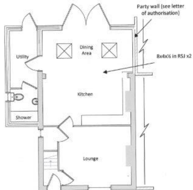
Proposed Ground Floor 1:100
