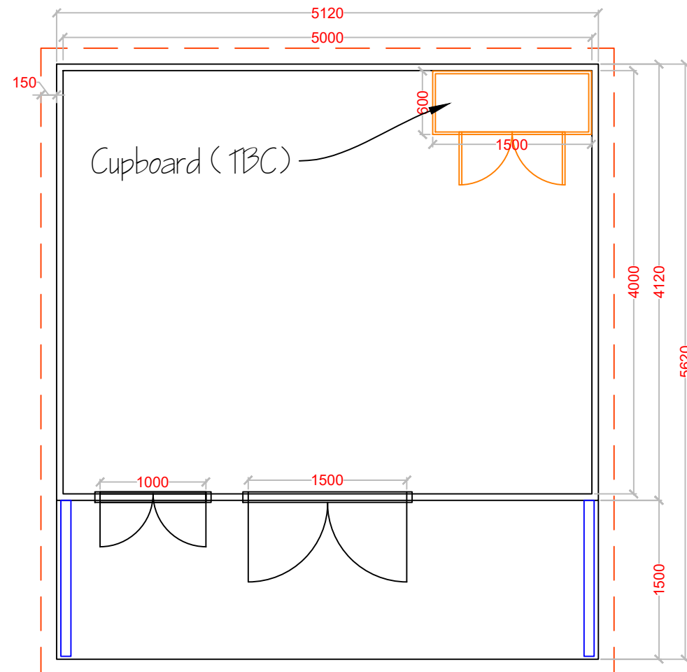
Layout Plan
