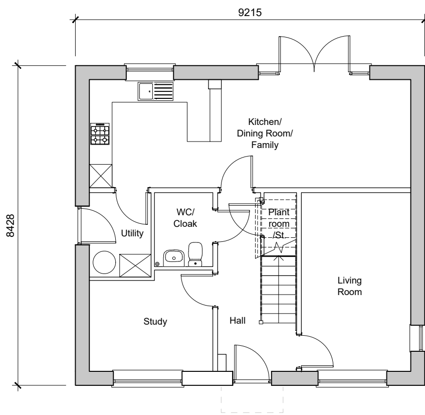
Ground Floor Plan 4-Bedroom House 130.46sqm / 1404.31sqft GIA (to be used) Plot - 173
