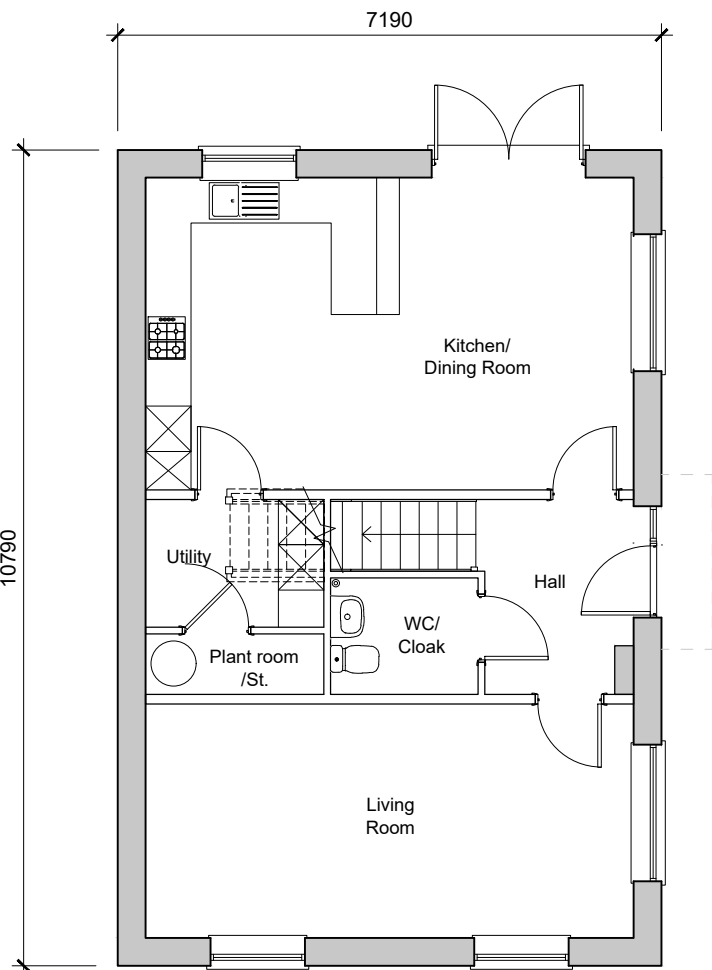
Ground Floor Plan 4-Bedroom House 129.8sqm / 1397sqft GFA (to finished) Plots - 66, 128
