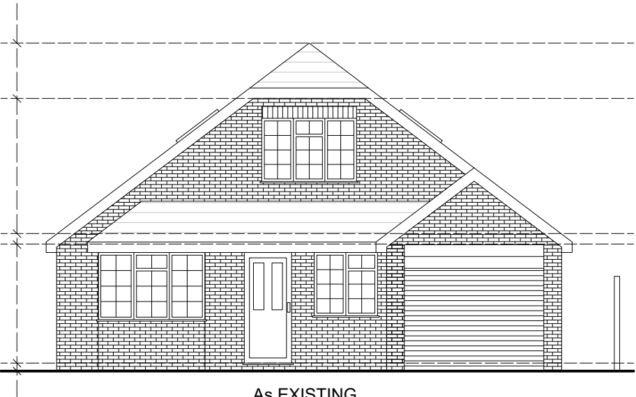
As EXISTING
