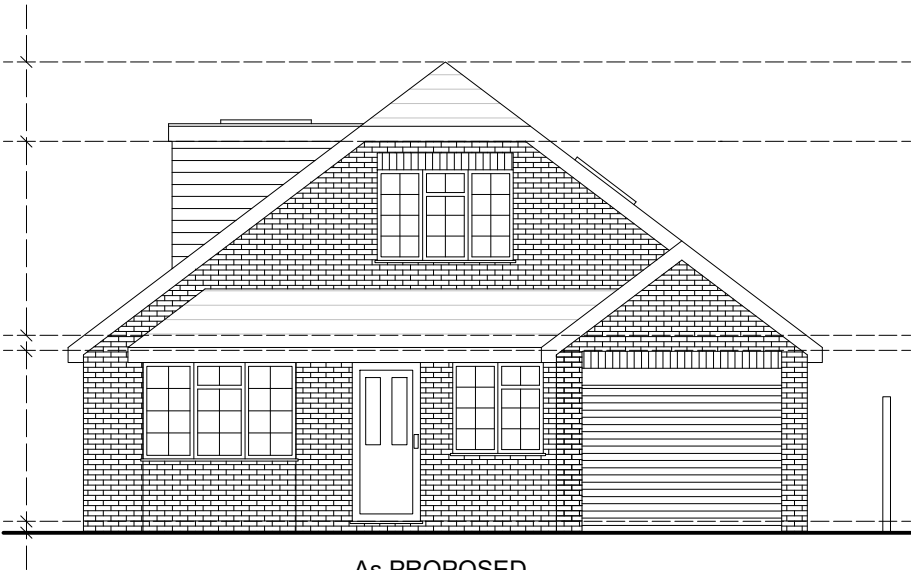
As PROPOSED
