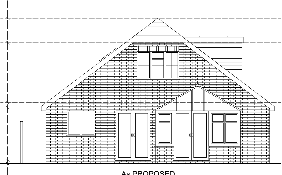
As PROPOSED
