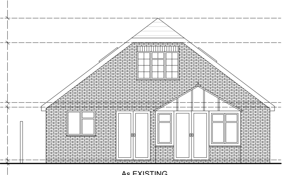
As EXISTING
