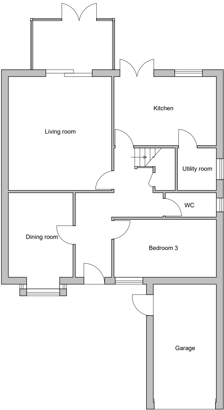
As EXISTING GROUND FLOOR PLANS
