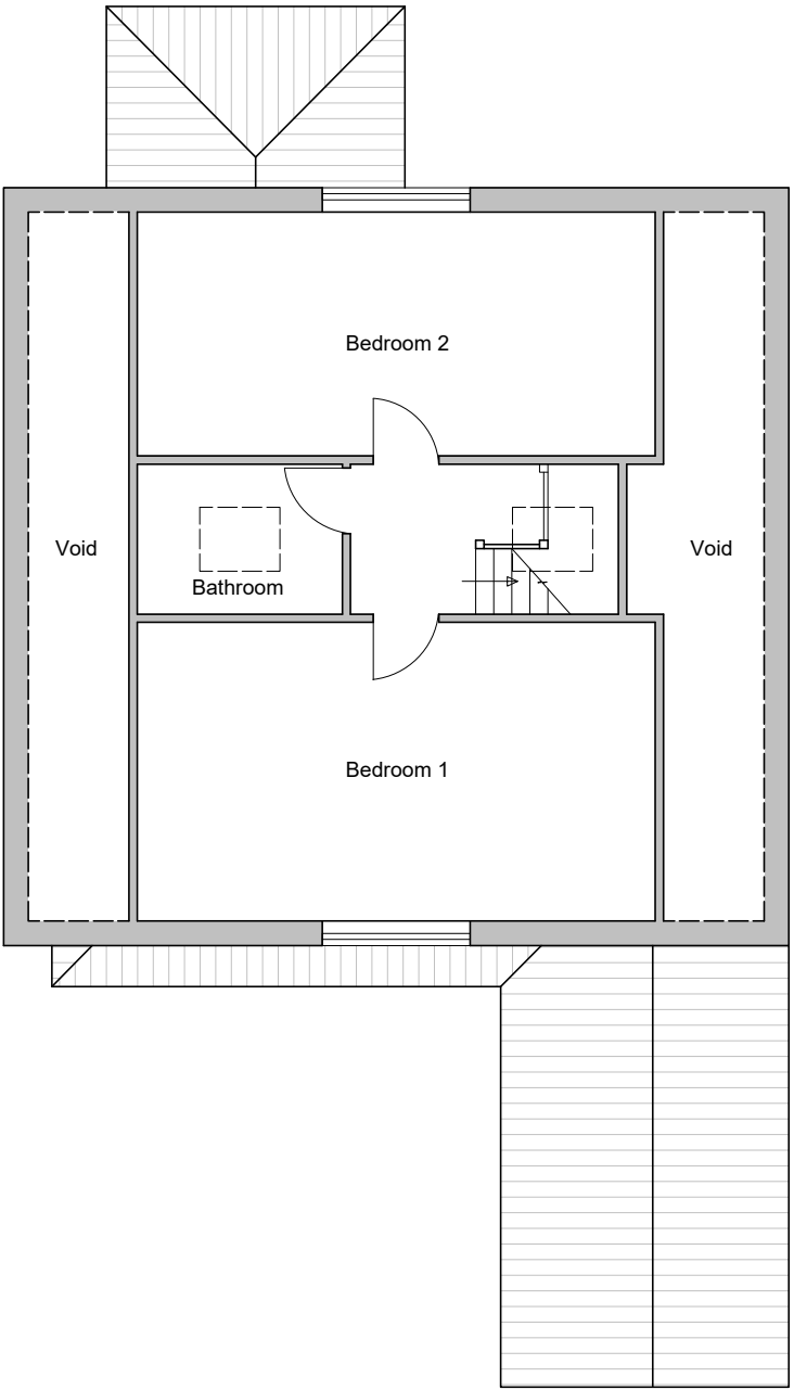
As EXISTING FIRST-FLOOR PLANS
