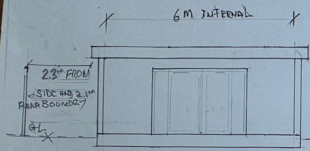
PROPOSED ELEVATION
