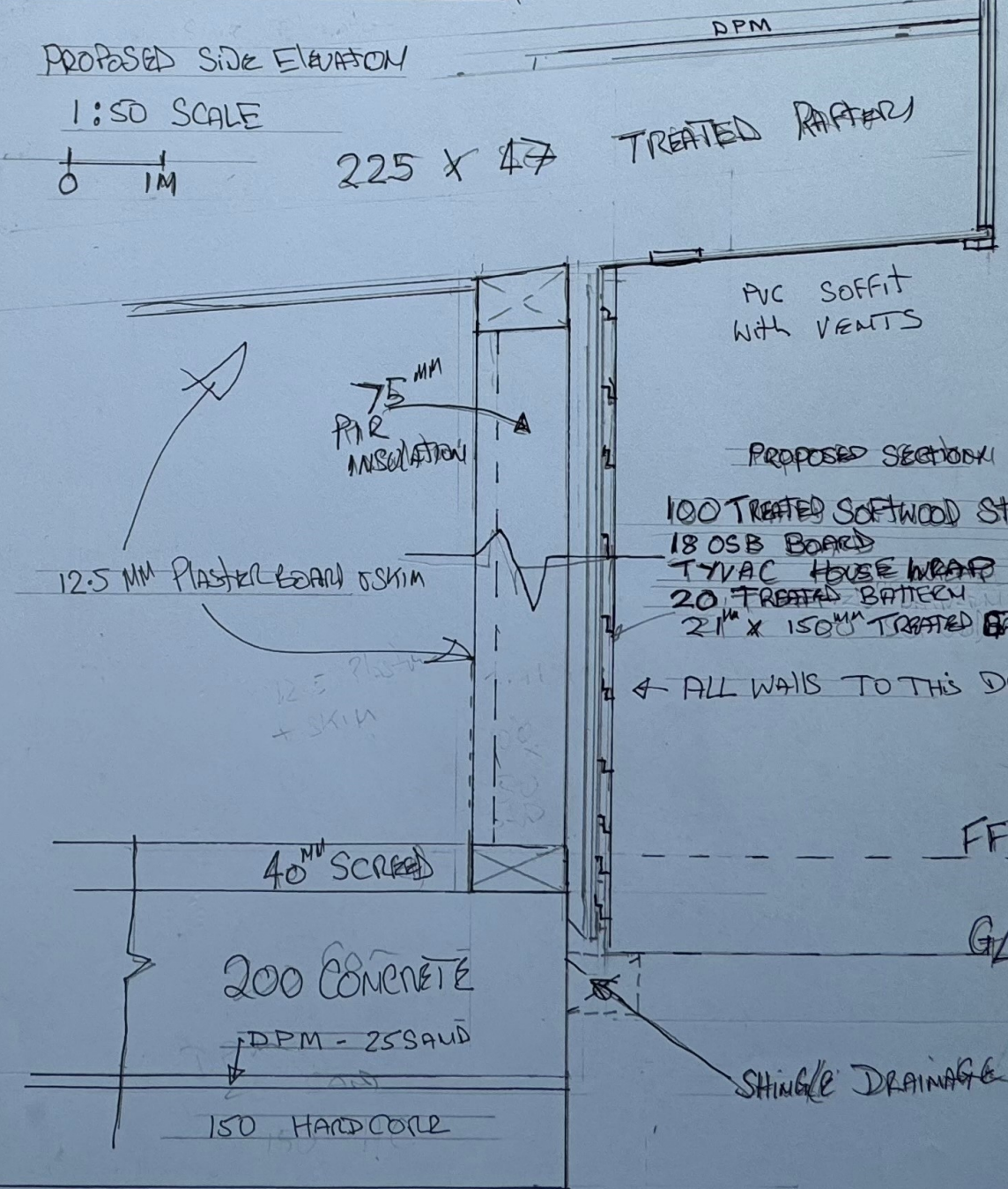
PROPOSED TYPICAL SECTION
