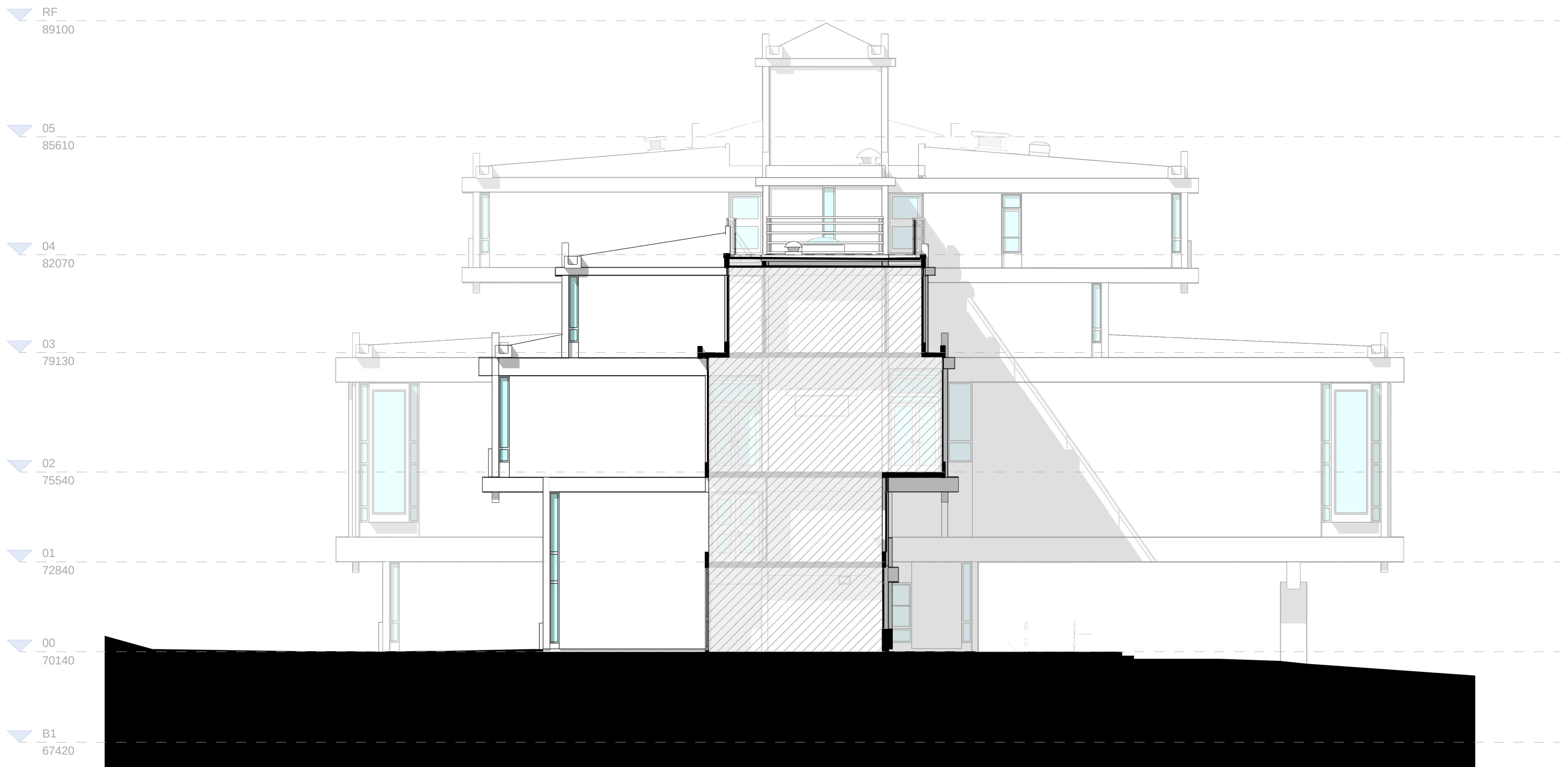
21003-Elevation-Cut-East_JJ_Existing 1:100
