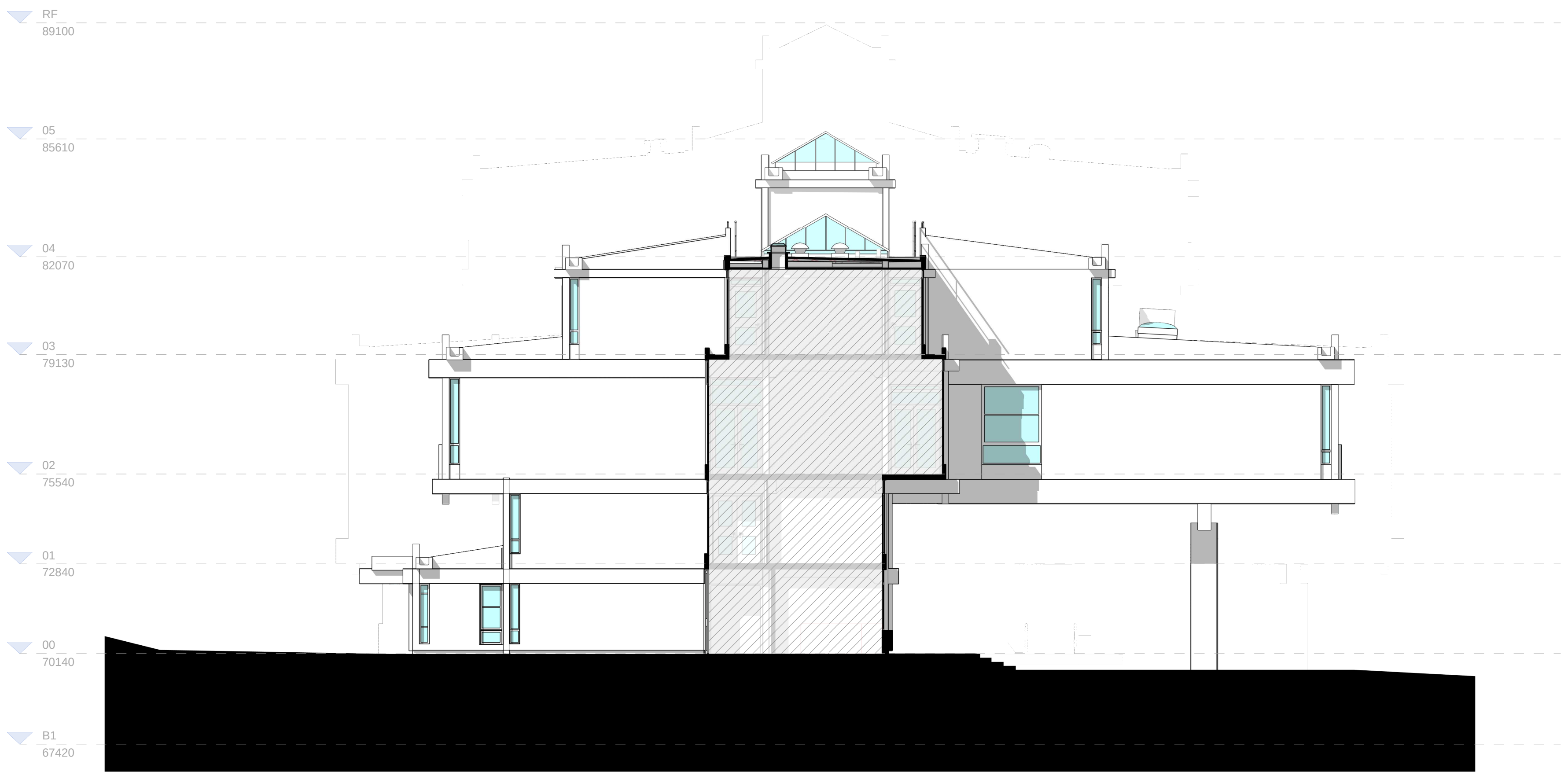
21003-Elevation-Cut-East_KK_Existing 1:100
