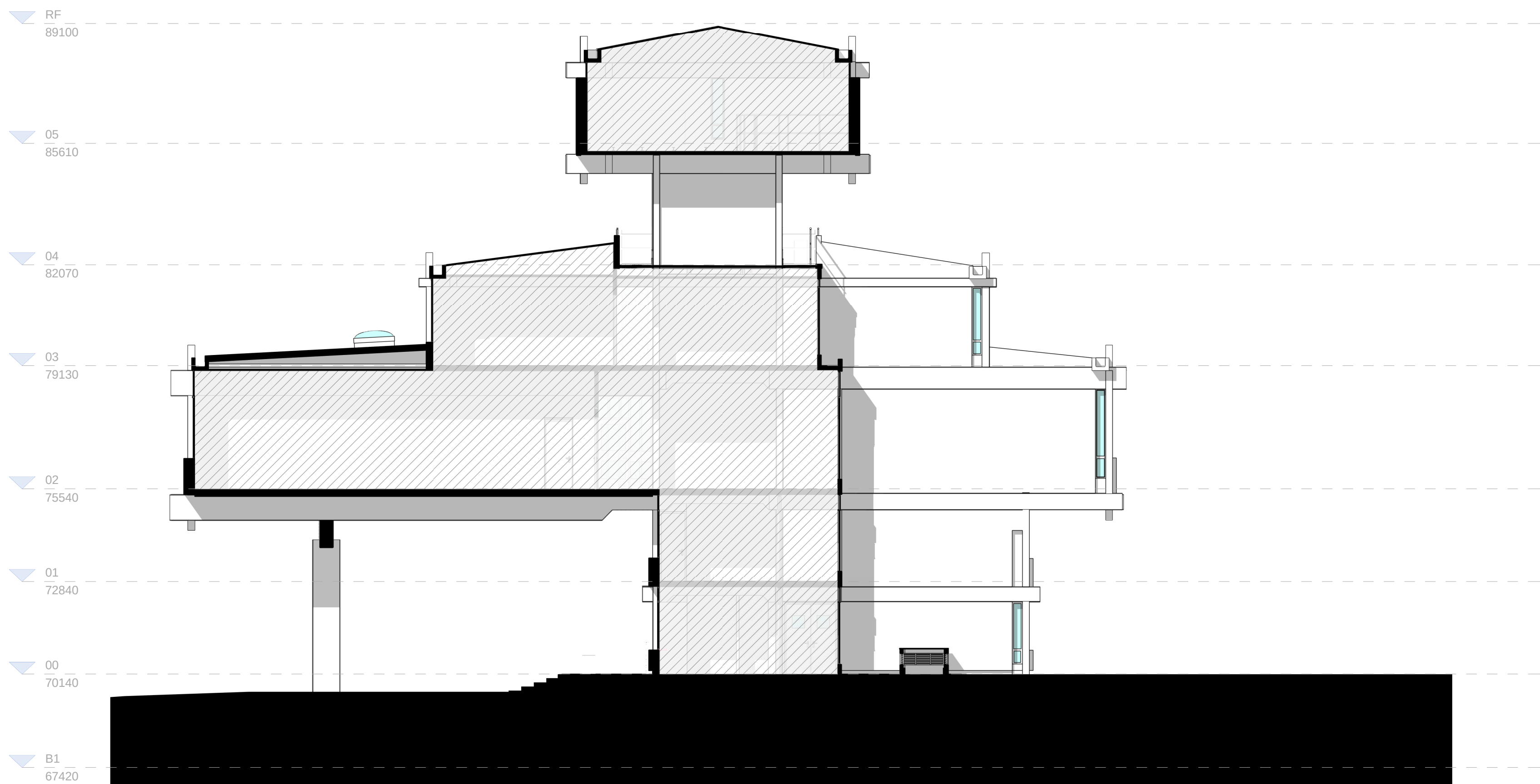
Q | 21005-Elevation-Cut-West_QQ_Existing 1:100
