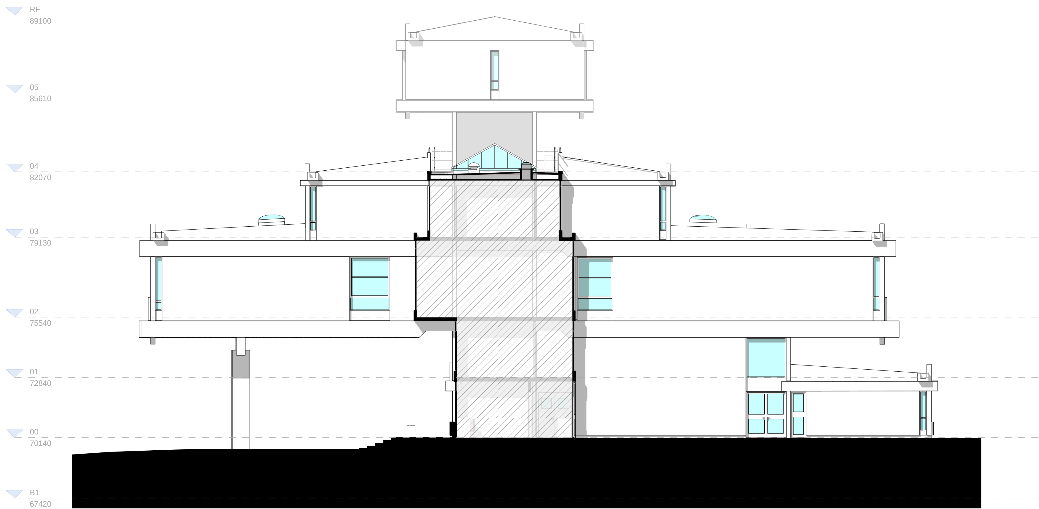
P | 21005-Elevation-Cut-West_PP_Existing 1:100
