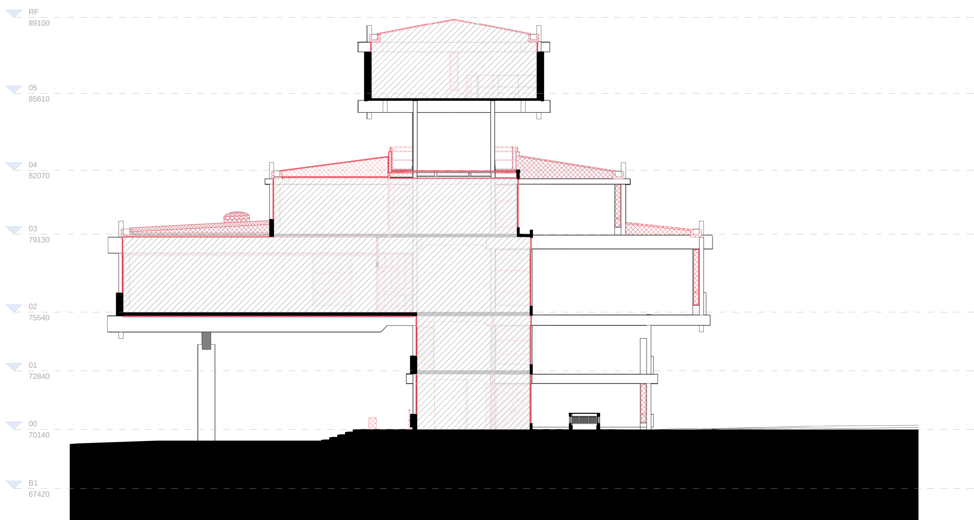
Q | 21135-Elevation-Cut-West_QQ_Phase3 1:100
