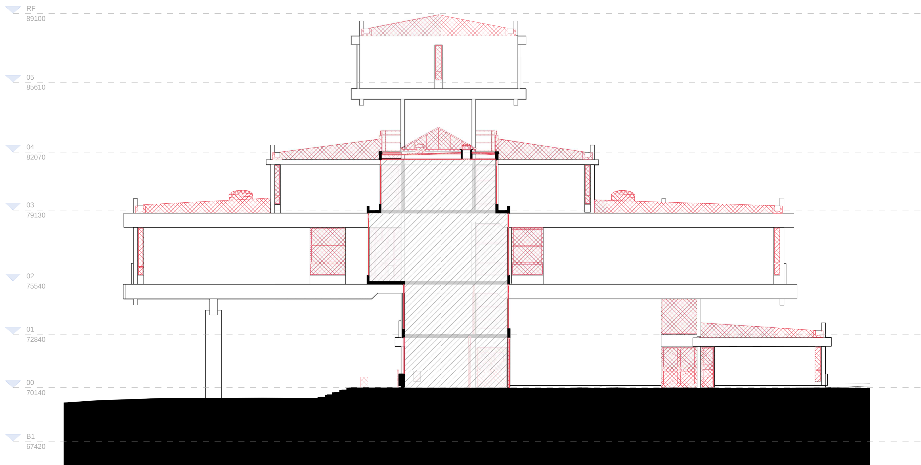
P | 21135-Elevation-Cut-West_PP_Phase3 1:100
