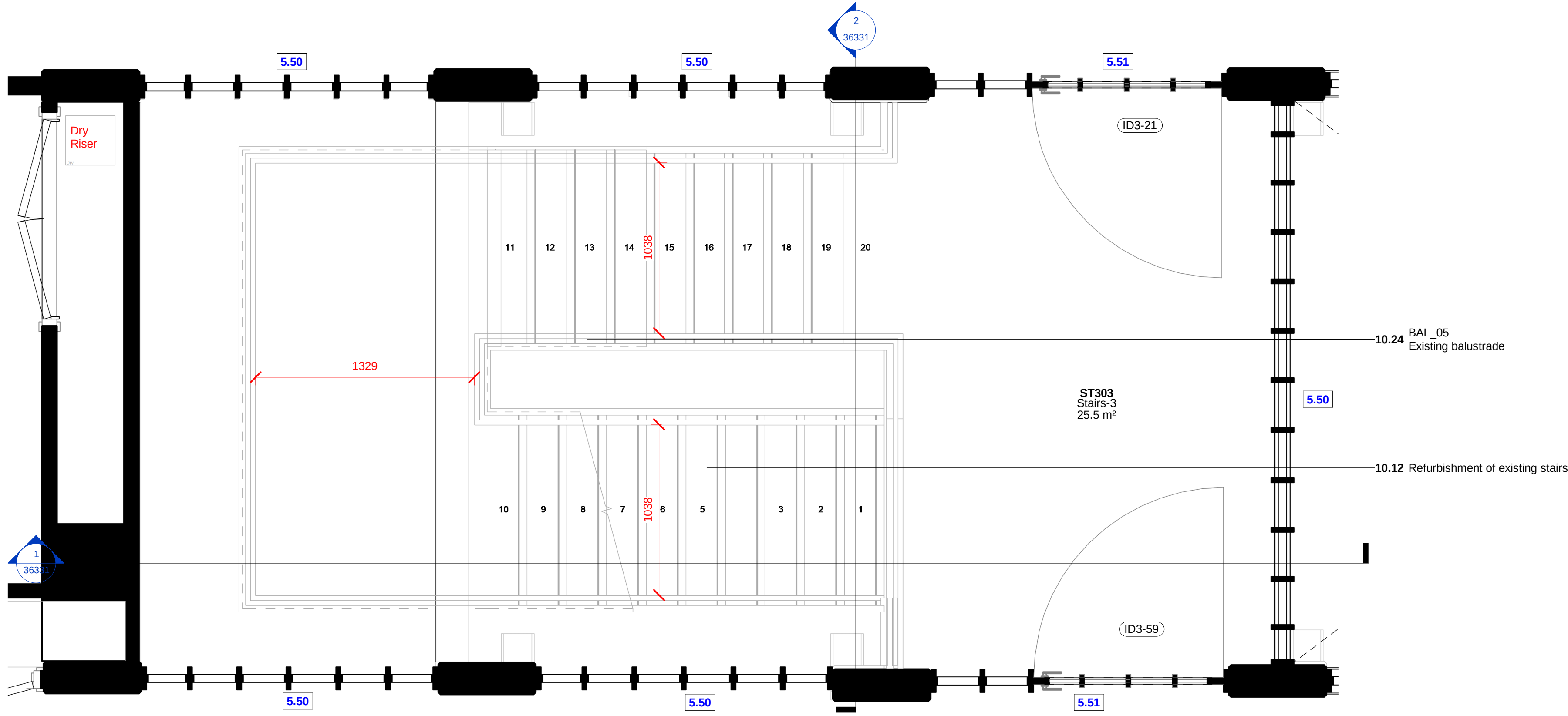
4 36330-Level 3 Plan
