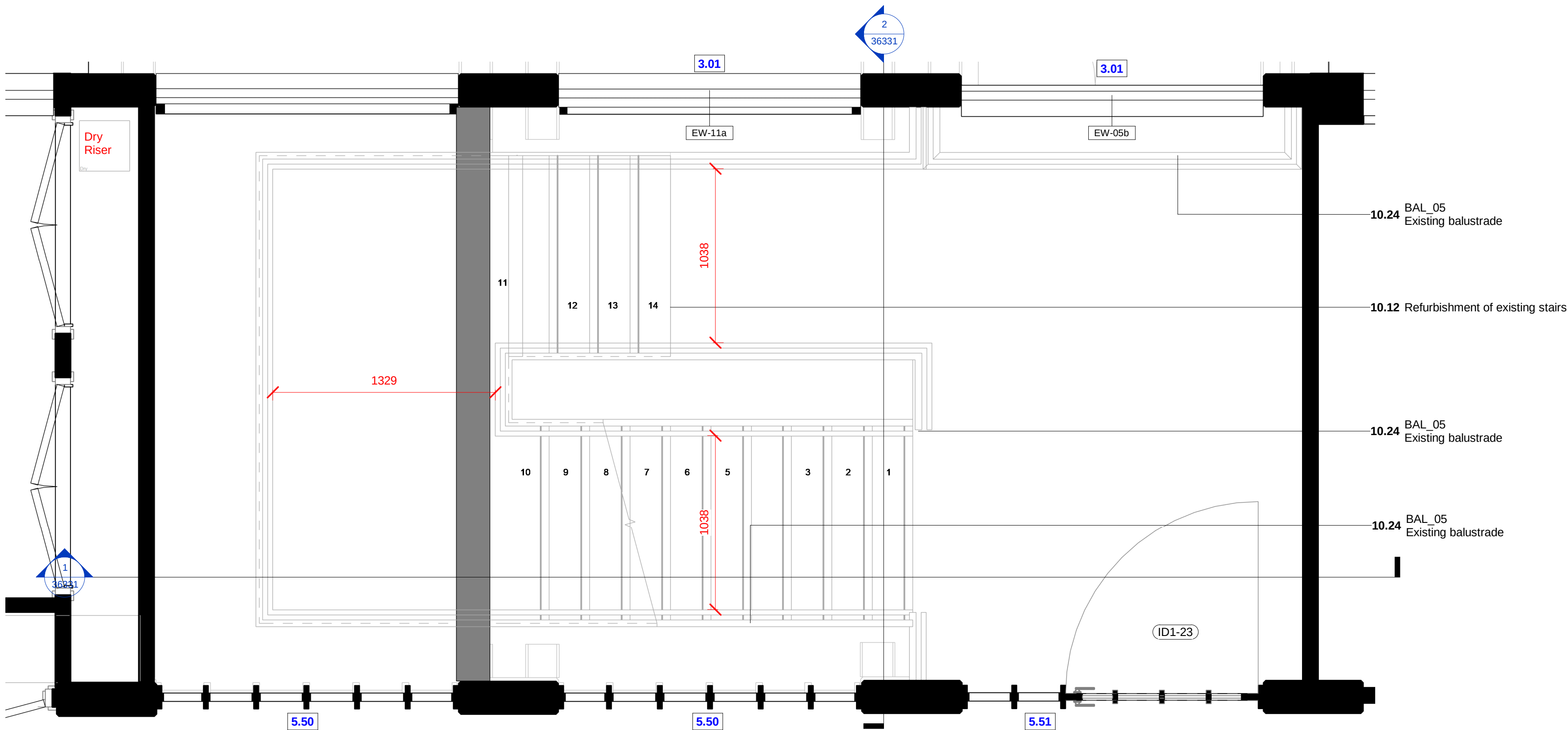
2 36330-level 1 Plan
