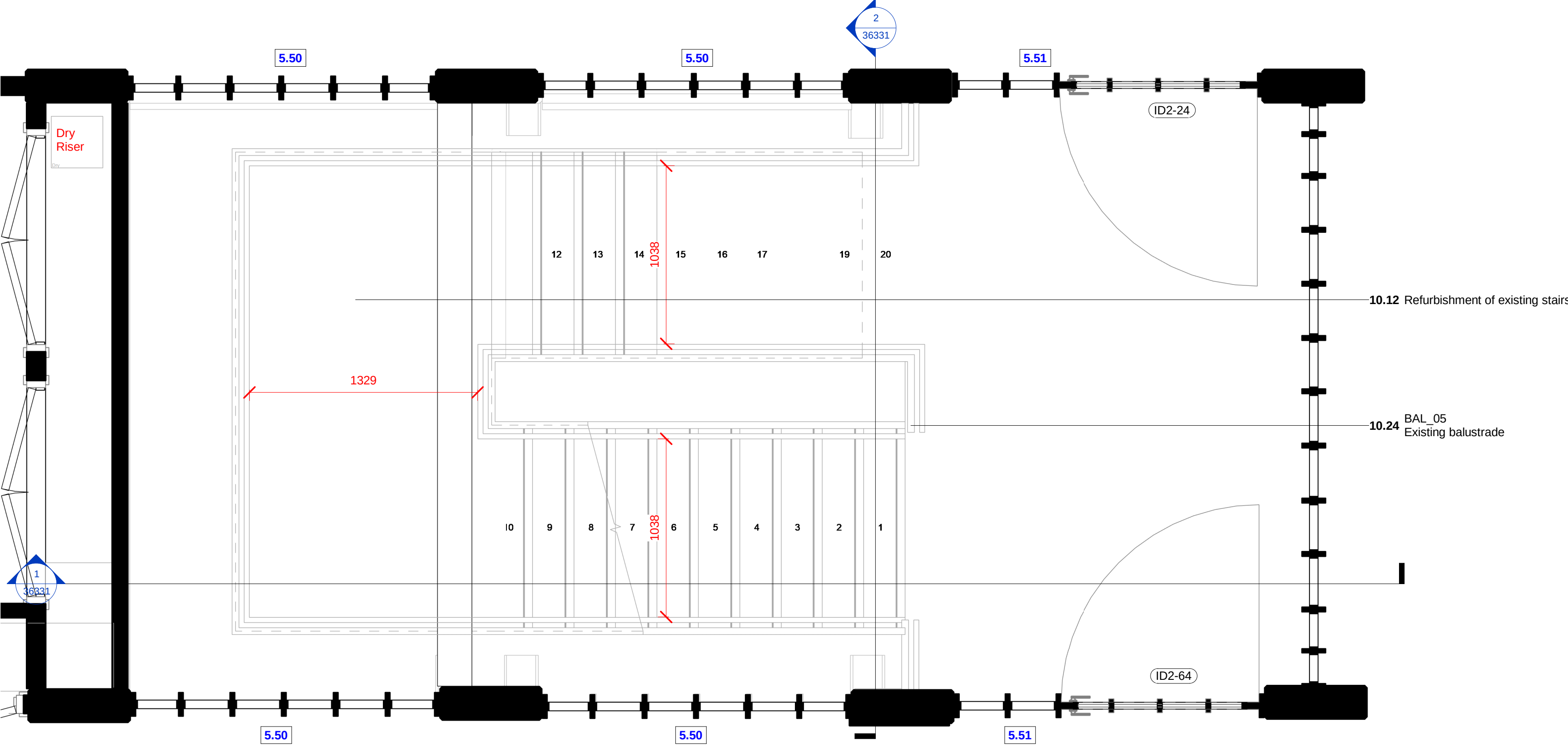
3 36330-Level 2 Plan
