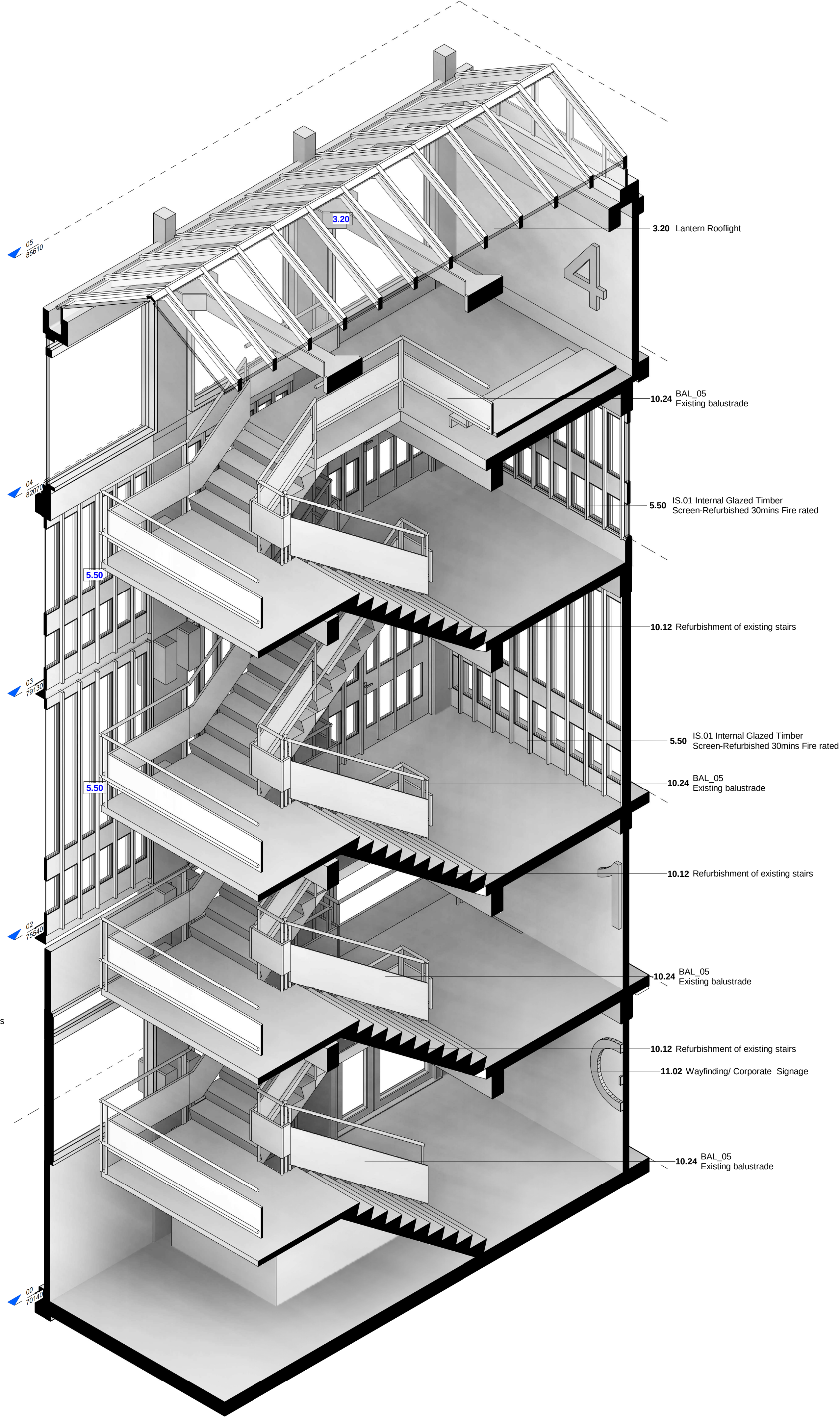
5 36310-3D View
