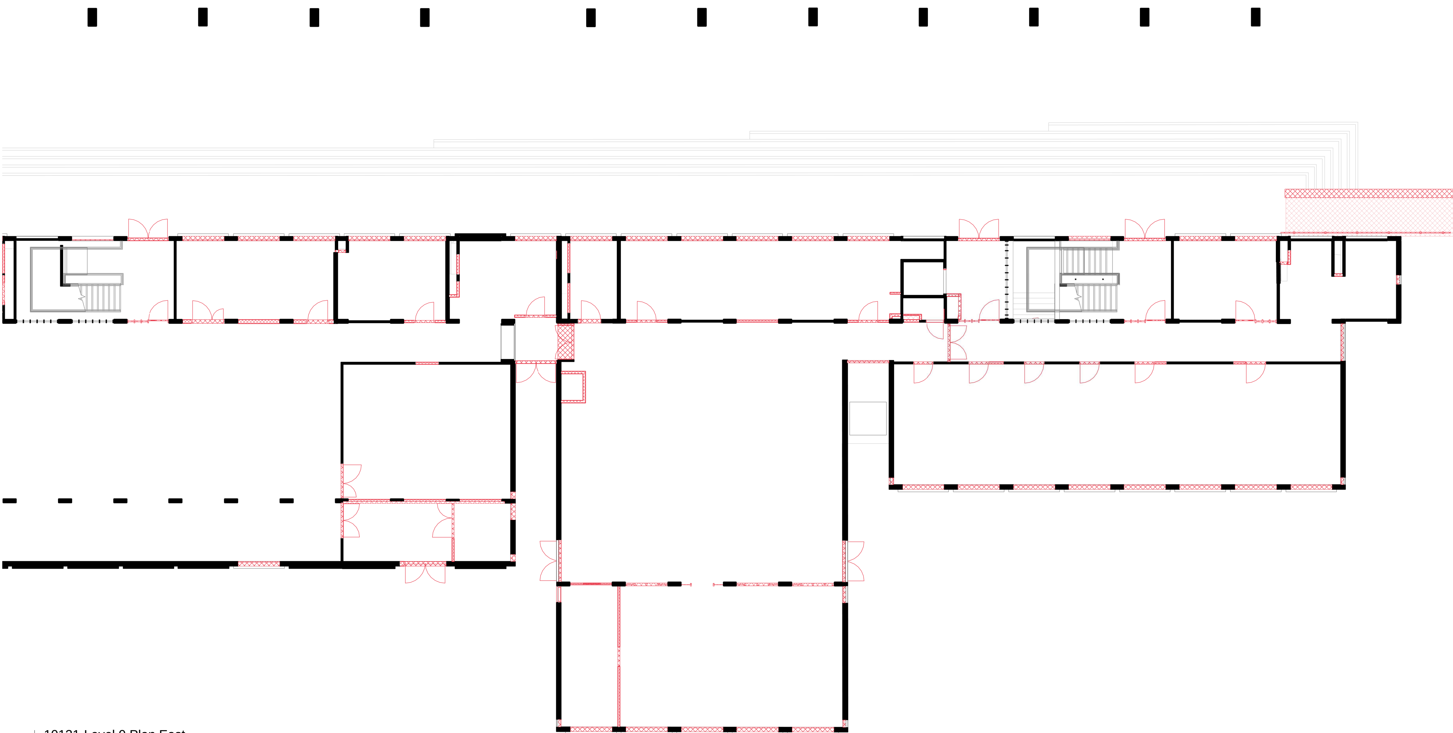
3 | 10131-Level 0 Plan East 1:100
