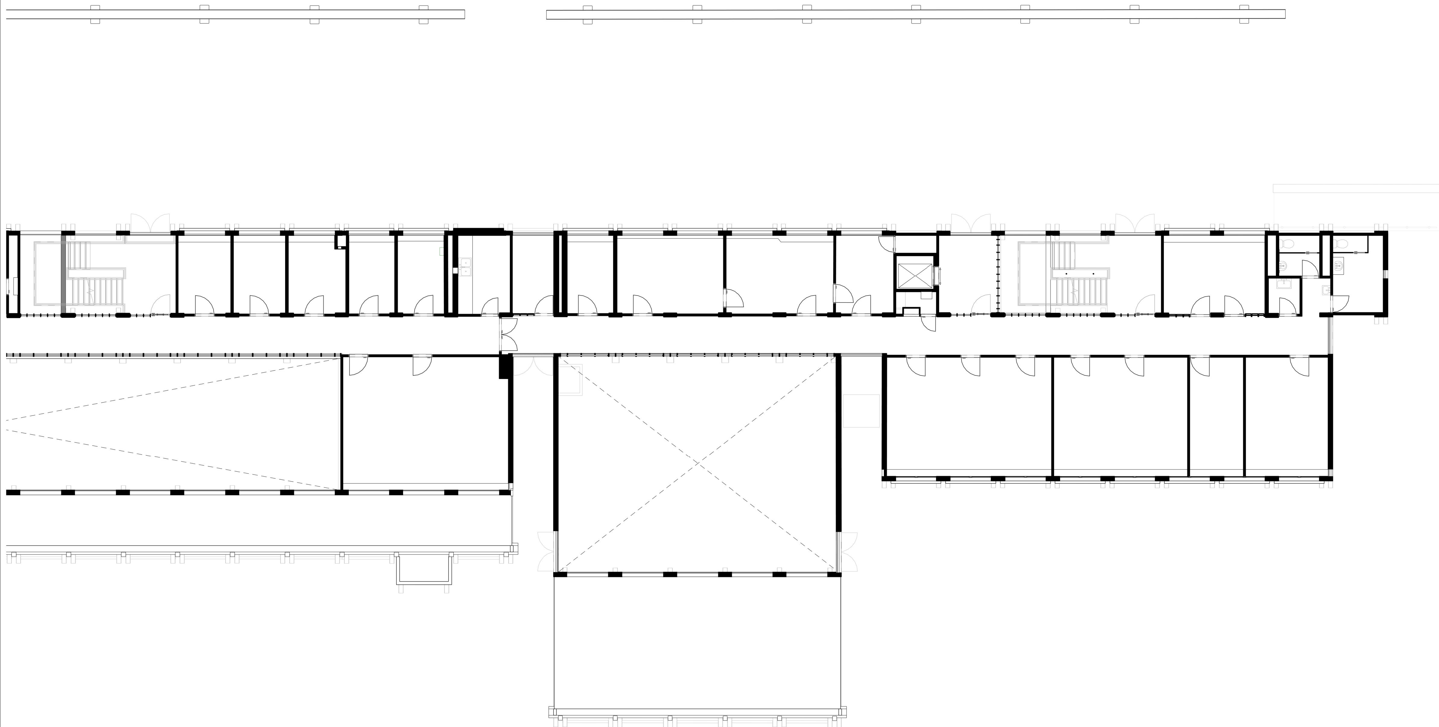
3 10011-Level 1 Plan East 1:100
