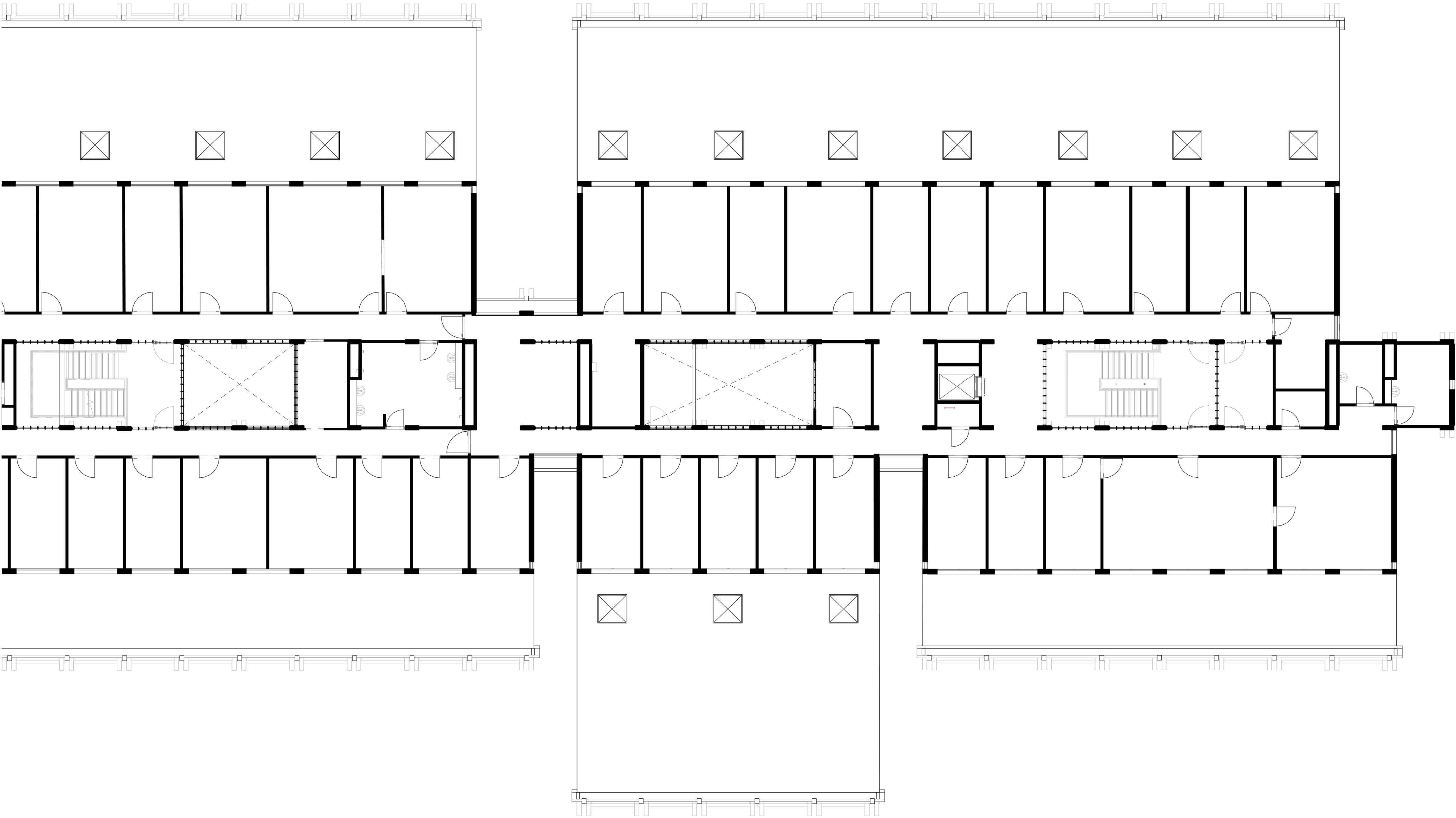
3 | 10013-Level 3 Plan East 1 : 100
