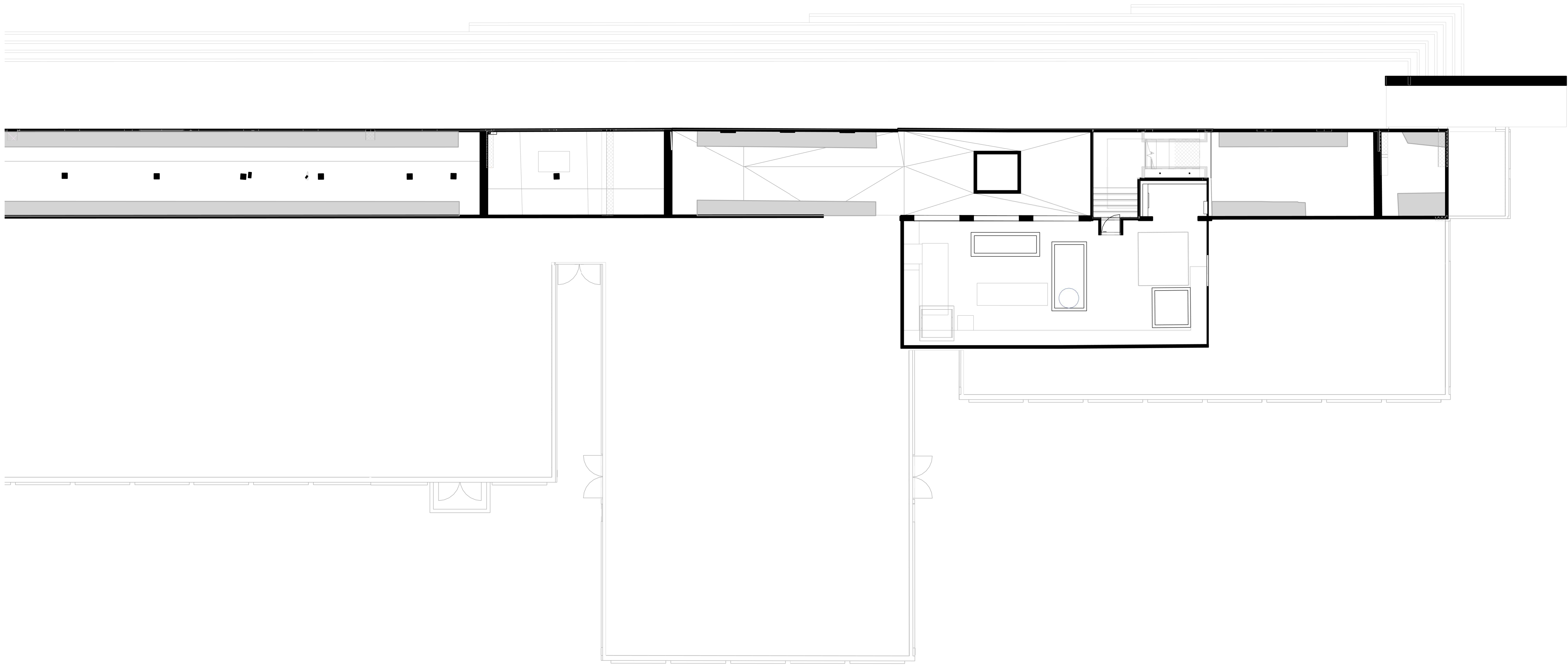
3 | 10016-Level B1 Plan East 1 : 100
