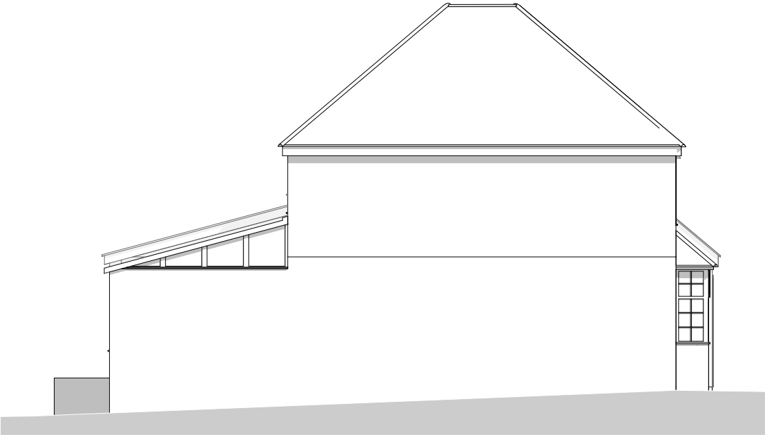
1:100 Existing Side Elevation
