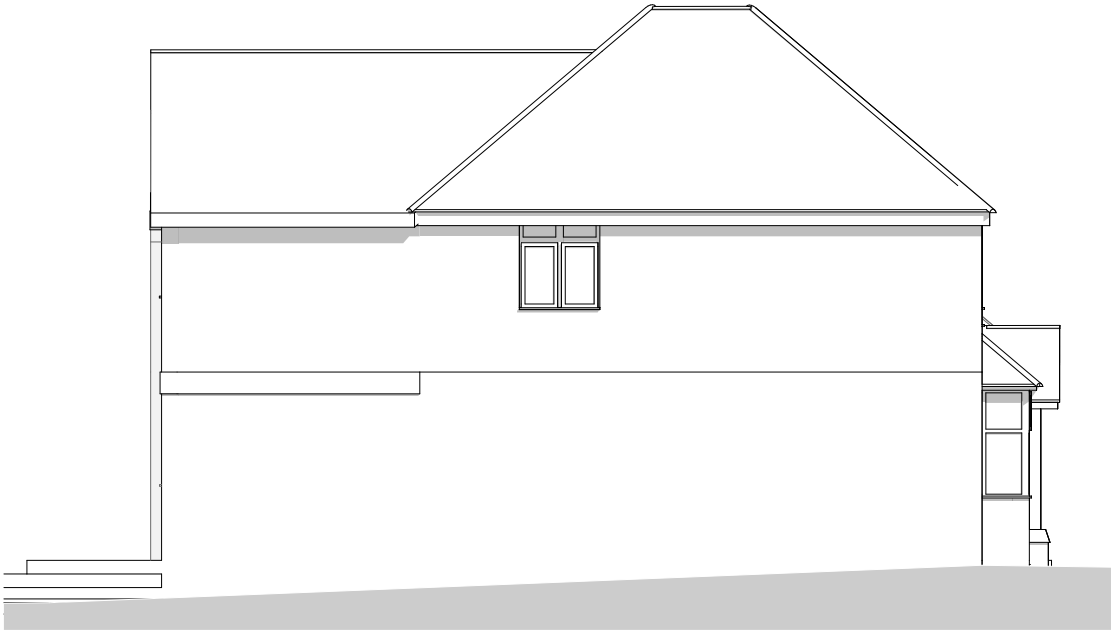
1:100 Proposed Side Elevation
