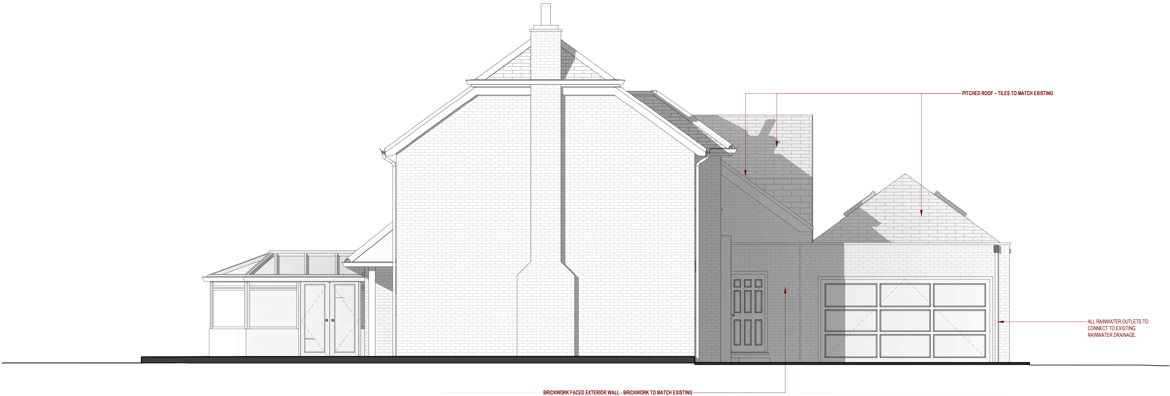
1 P03. PROPOSED SIDE ELEVATION 1:50
