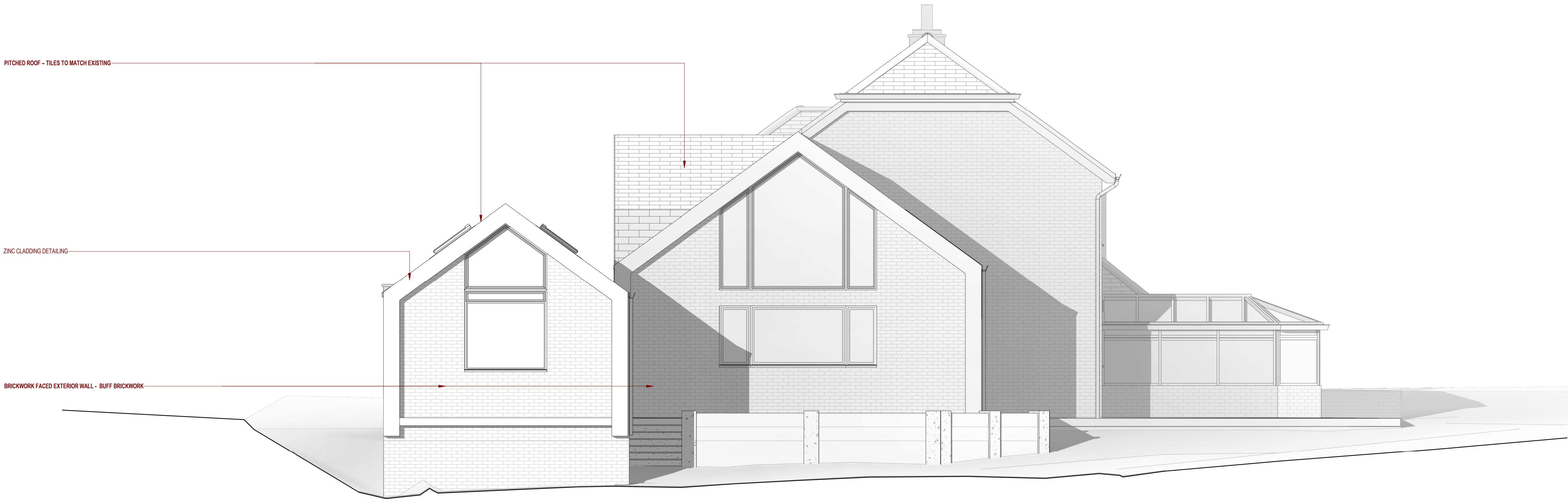
2 P04. PROPOSED SIDE ELEVATION 1:50
