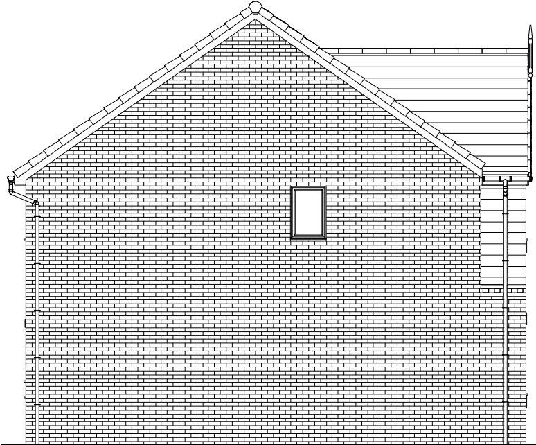
REAR
