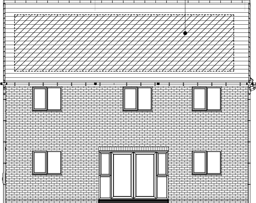
REAR
