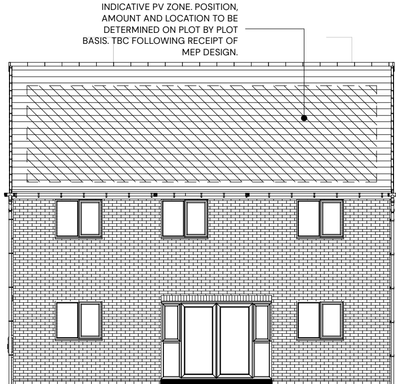
REAR
