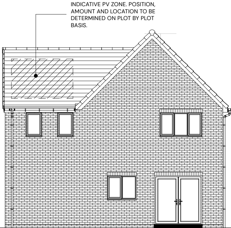
REAR
