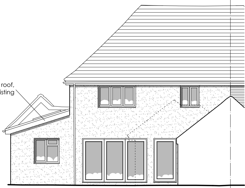
REAR ELEVATION 1:100
