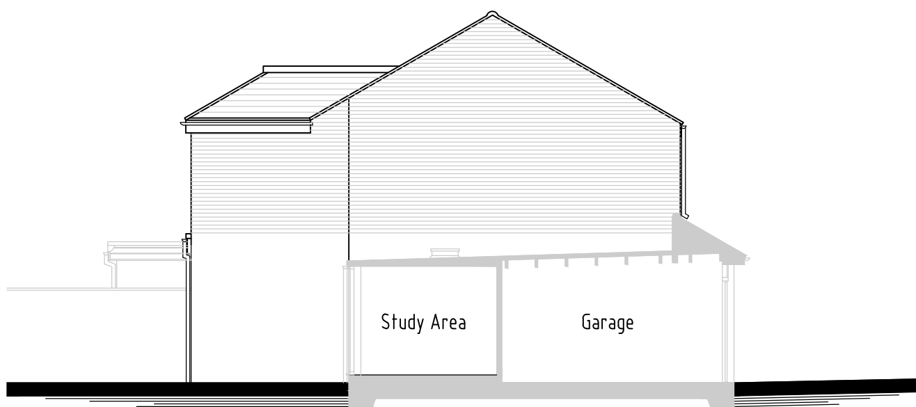
PROPOSED SOUTH ELEVATION - SECTION B-B
