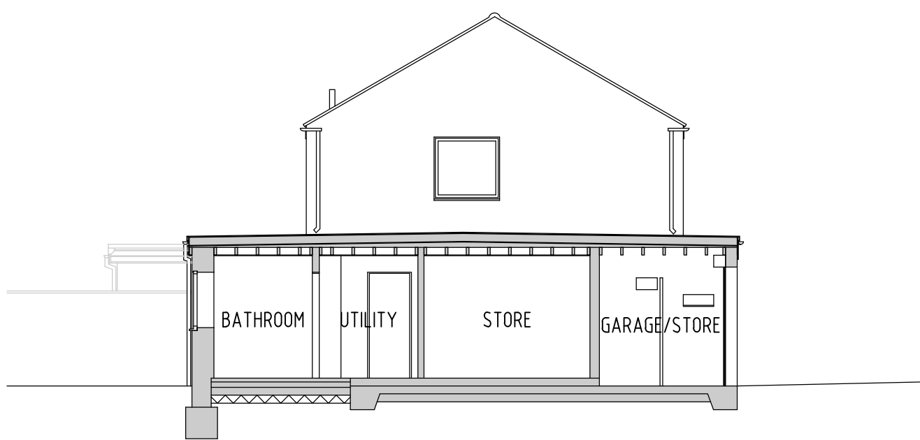
EXISTING SOUTH ELEVATION - SECTION B-B
