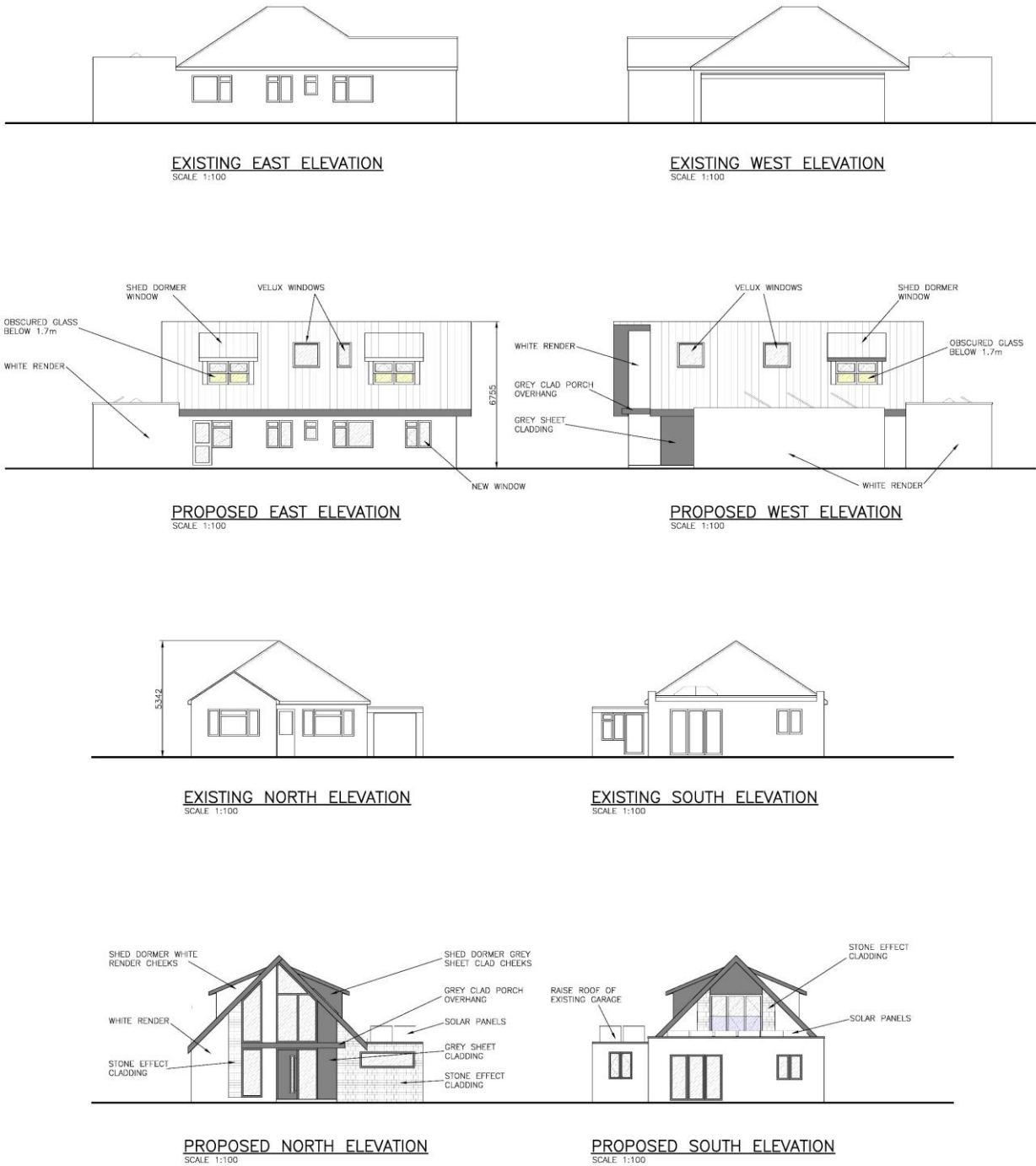
Figure 2 – Existing and proposed elevations
