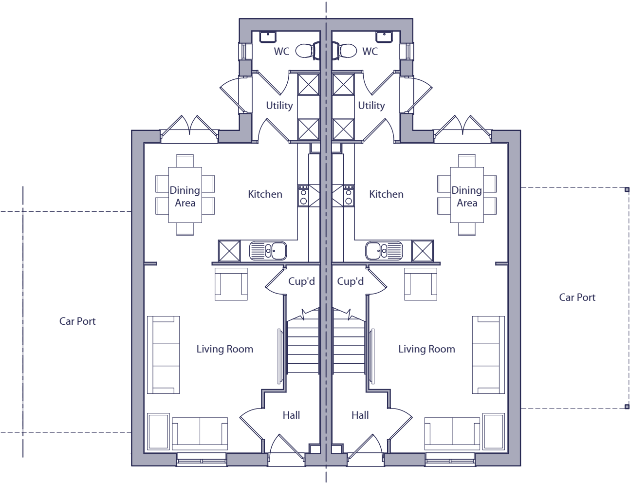
GROUND FLOOR PLAN PLOT 4027
