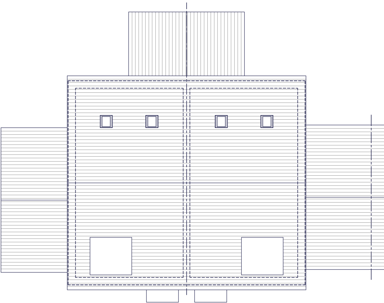
ROOF PLAN
