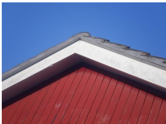
Photograph 5. Intact verge mortar and timber cladding on front gable (southern elevation).
