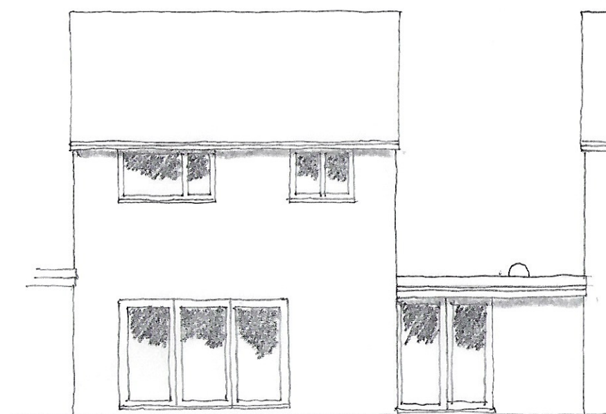
REAR ELEVATION 1:100
