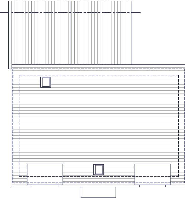
ROOF PLAN
