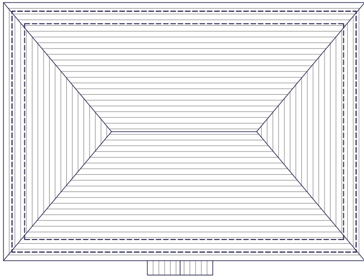
ROOF PLAN
