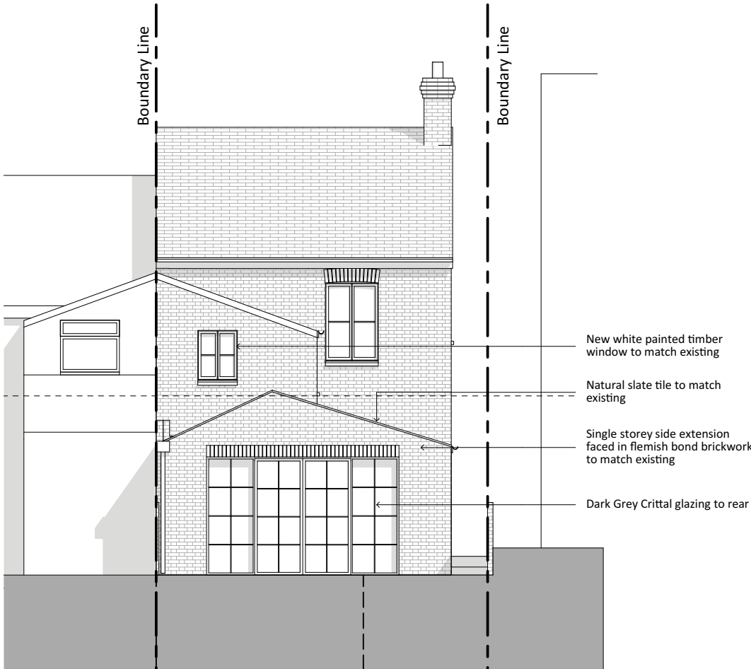
North Elevation
