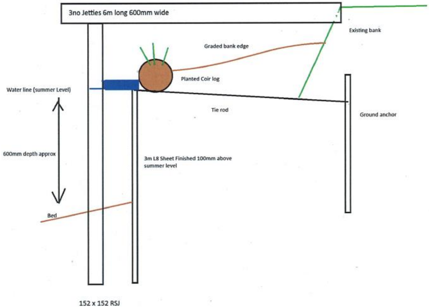
Low level Piling Detail
