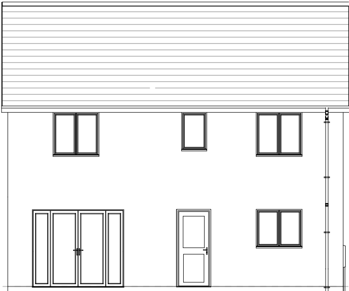
REAR ELEVATION
