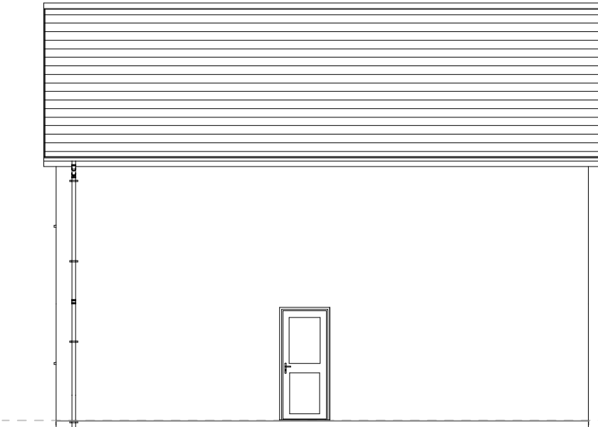
REAR ELEVATION
