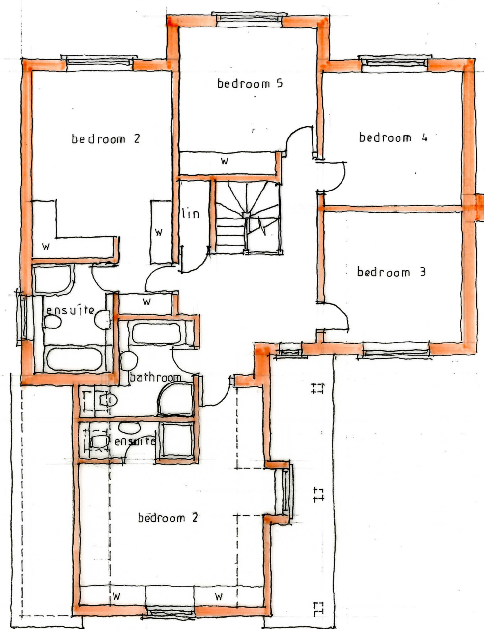
FIRST FLOOR
