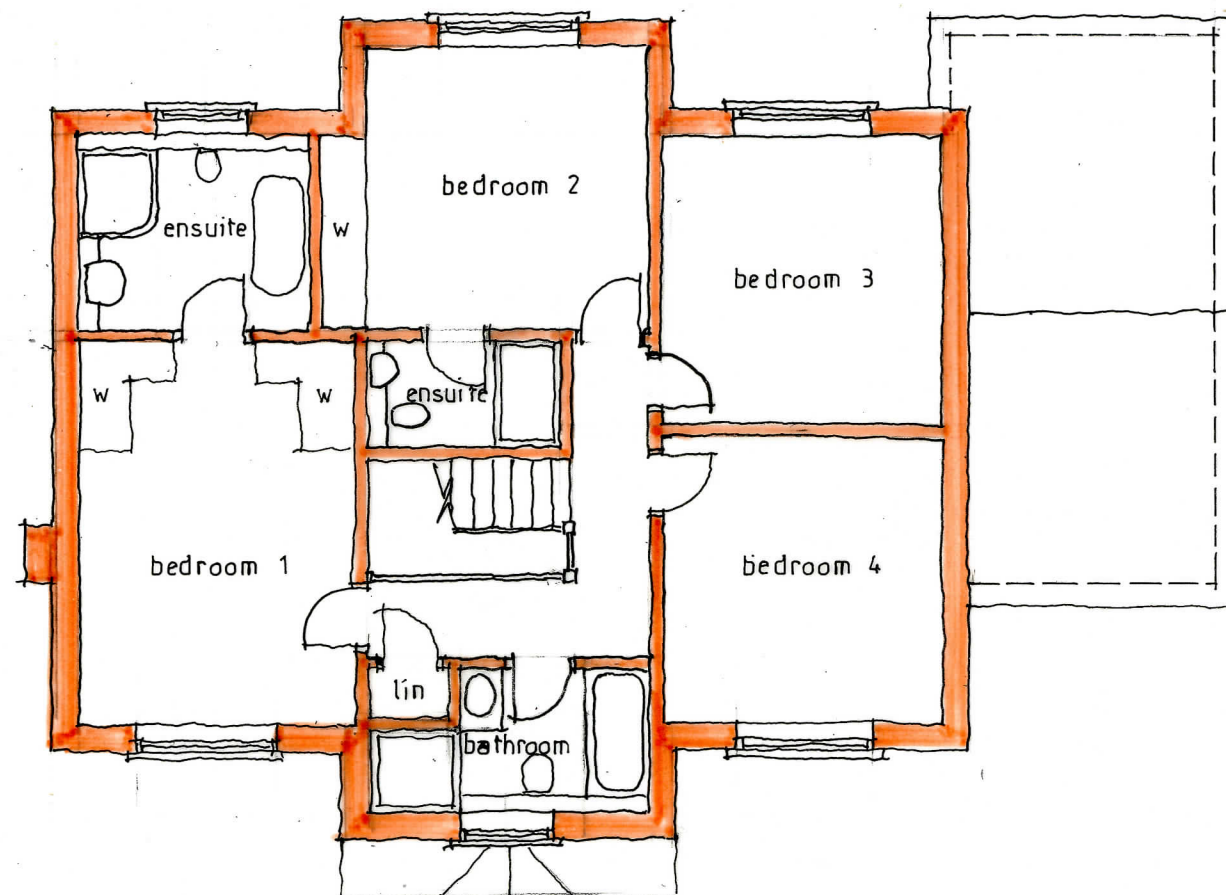
FIRST FLOOR
