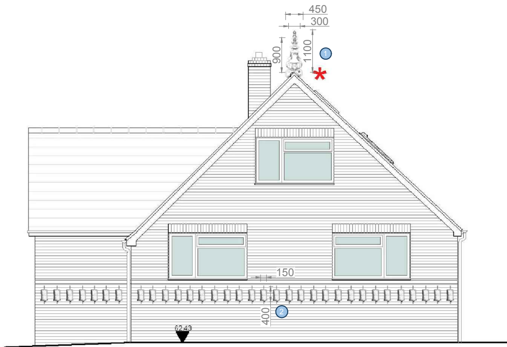
Proposed Side Elevation (South)
