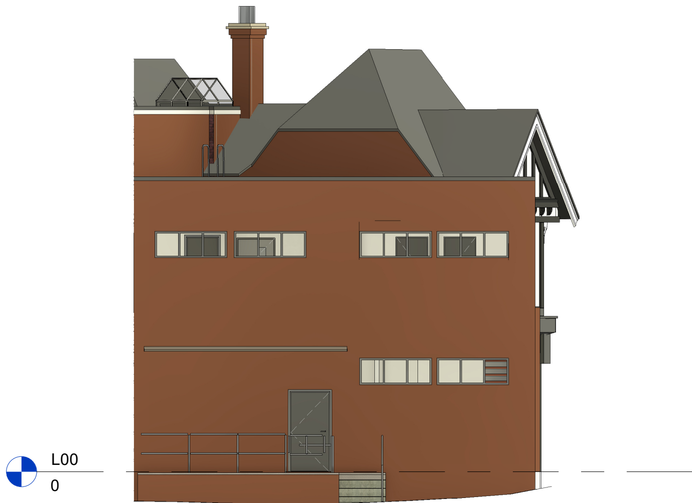
Prop. Rear Elevation 1 : 100
