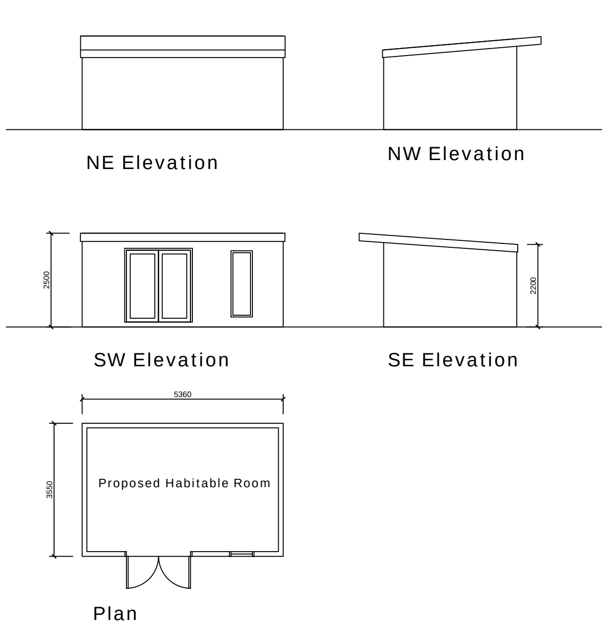
Existing 1:100 Plan and Elevations
