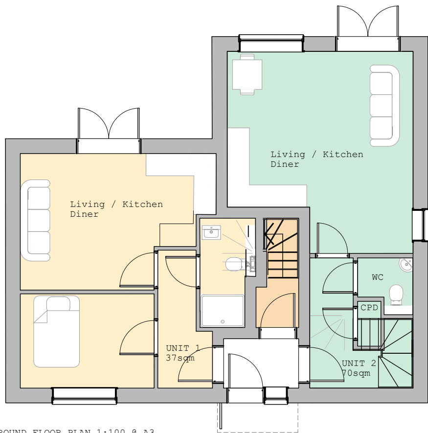
GROUND FLOOR PLAN 1:100 @ A3
