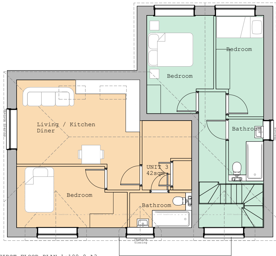
FIRST FLOOR PLAN 1:100 @ A3
