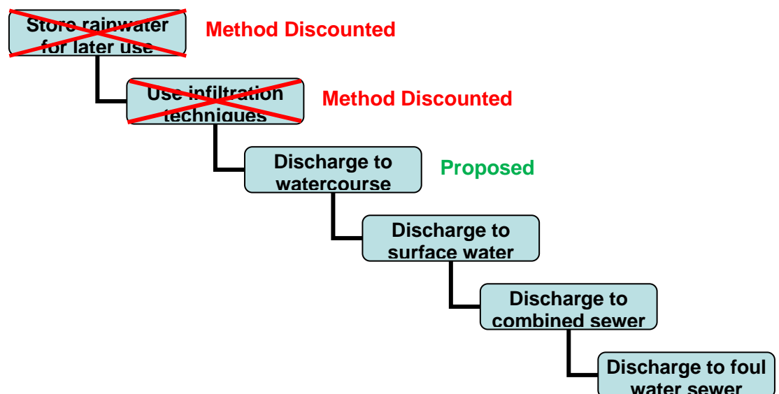
Figure 8.1 – SuDS Hierarchy
