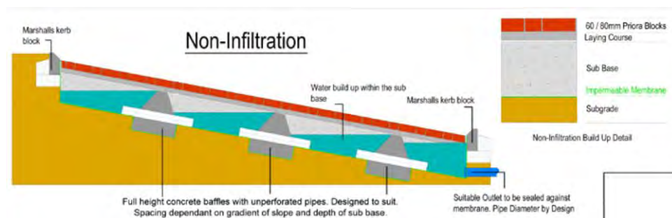
Figure 8.2 – Permeable Paving on Sloping Site.
