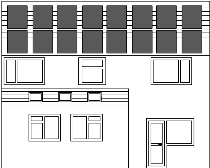
Rear Elevation
