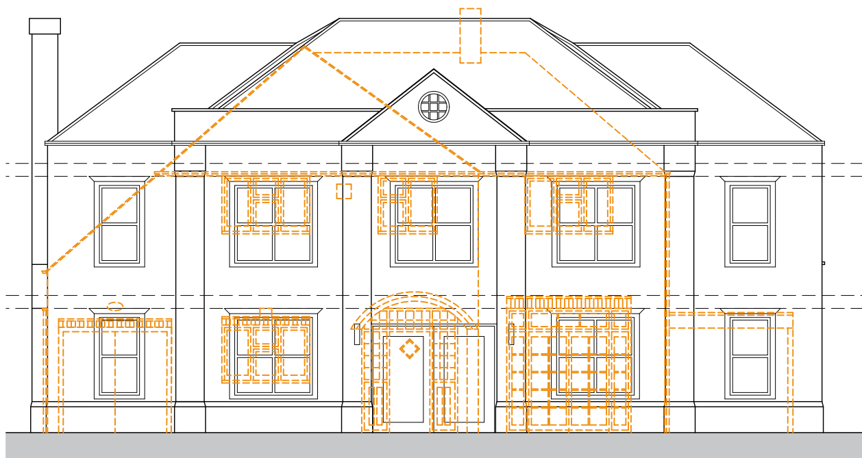
FRONT (SOUTH) ELEVATION
