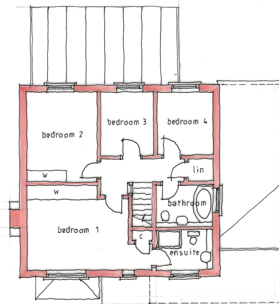
FIRST FLOOR
