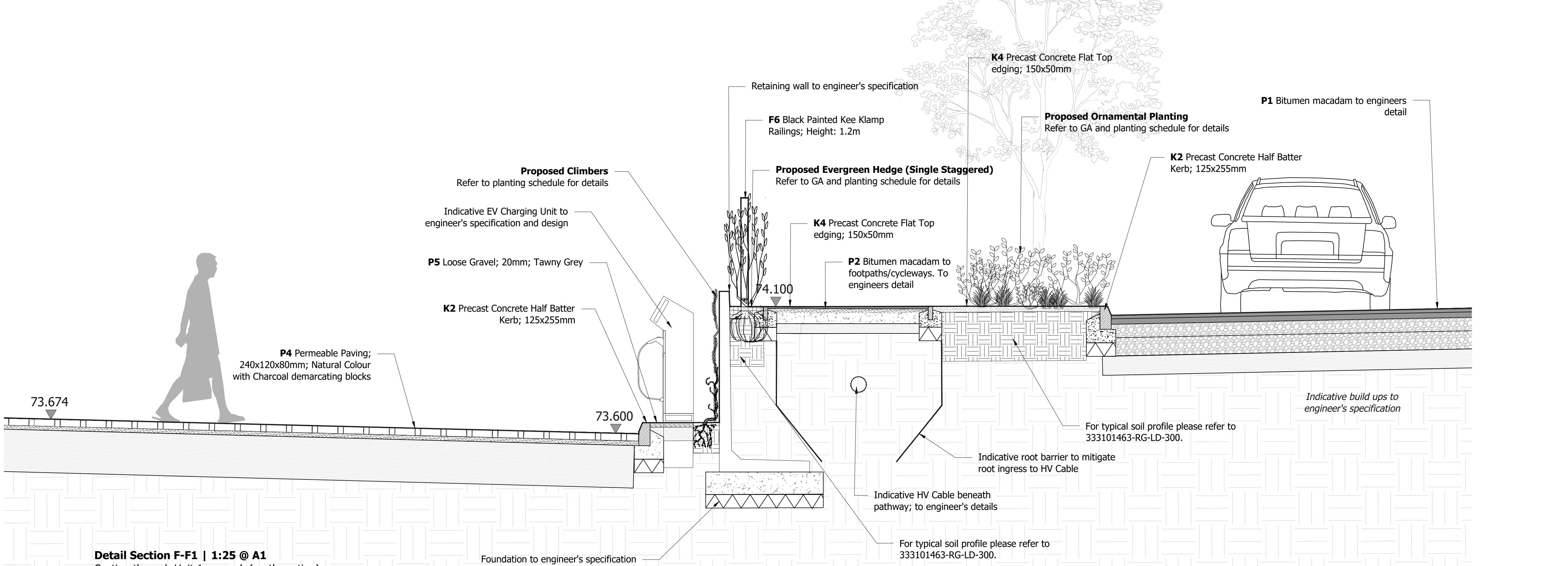
Detail Section F-F1 | 1:25 @ A1 Section through Unit 1 car park (north section) towards access road
