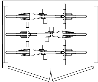
CYCLE STORE - Plan (1:50)
