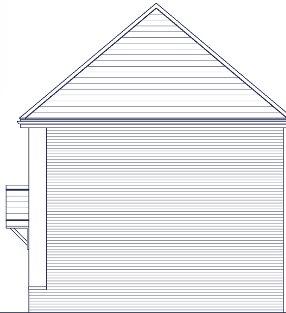
SIDE ELEVATION
