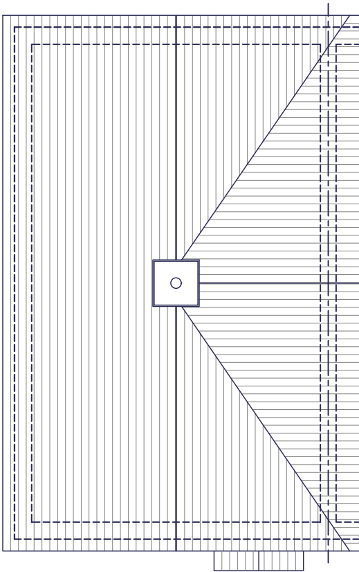
ROOF PLAN
