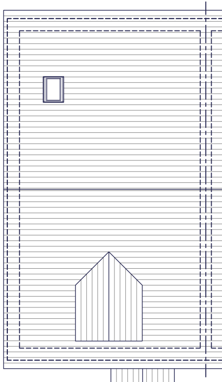
ROOF PLAN
