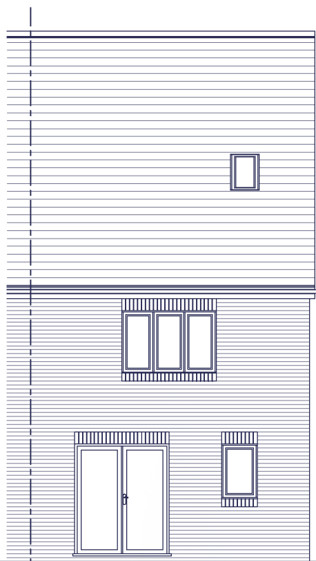
REAR ELEVATION
